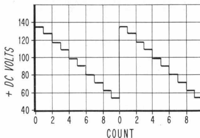
Fig. 3(b). Explanatory drawing indicating voltage excursion and count relation. Plateaus correspond to counts.
